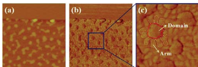
Figure 5. (a) AFM height image of the BCCP Langmuir monolayer obtained after scratching off the top portion of monolayer. Scan size = 1 \mu\text{m} \times 1 \mu\text{m} and z scale = 50 nm. (b) The corresponding phase image of (a). Phase scale = 50^\circ . (c) Close-up of the phase image in (b); the domain is enclosed with red dash line and arms with white. Scan size = 0.3 \mu\text{m} \times 0.3 \mu\text{m} and phase scale = 50^\circ . The original Langmuir monolayer was obtained at \pi = 5 \text{ mN/m} .
