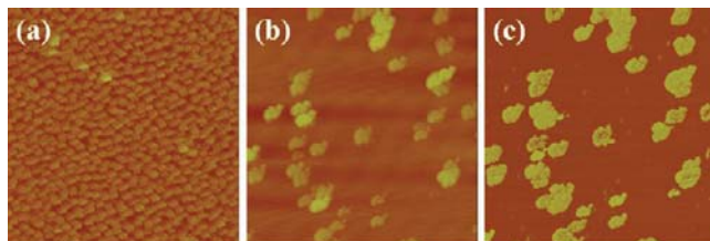
Figure 8. (a) AFM height image of Langmuir monolayer after immersion in the buffer solution without the addition of enzyme for 1 h. (b) AFM height image of Langmuir monolayer undergoing enzymatic degradation for 1 h. (c) Corresponding phase image of (b). Scan size = 3 \mu\text{m} \times 3 \mu\text{m} , z scale = 50 nm, and phase scale = 50^\circ . The original Langmuir monolayer was obtained at \pi = 5 \text{ mN/m} .
